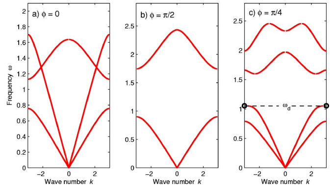
FIG. 14. (Color online). Dispersion relation \omega(k) of the periodic stack in Fig. 6 for three different values of the misalignment angle \phi . In the cases \phi=0 (no misalignment) and \phi=\pi/2 , none of the spectral branches can develop a degenerate band edge (DBE). While in the case (c) of \phi=\pi/4 , one of the spectral branches develops a DBE.
