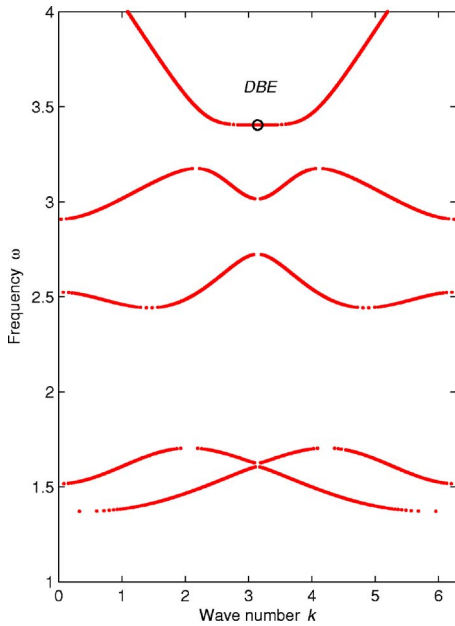
FIG. 16. (Color online) Axial dispersion relation \omega(k_z) of the two-layered periodic stack in Fig. 8. The tangential components k_x, k_y of the wave vector are fixed at k_x=k_y=1.9403 . The fifth spectral branch develops a degenerate band edge (45) at k_z=\pi/L .
