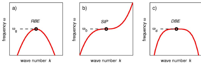
FIG. 2. (Color online) Schematic examples of dispersion relations displaying different stationary points: (a) a regular band edge (RBE), (b) a stationary inflection point (SIP), (c) a degenerate band edge (DBE).
