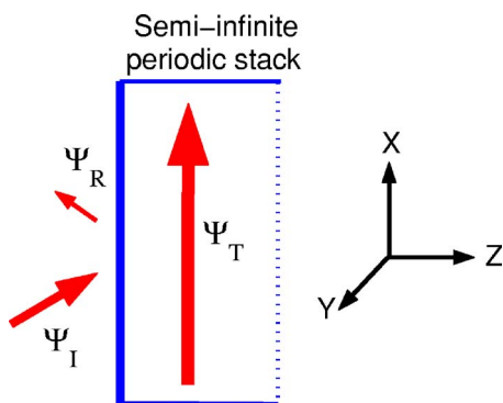
FIG. 13. (Color online) The case of oblique incidence, where the transmitted wave is a grazing mode with tangential energy flux and a frozen mode profile.
