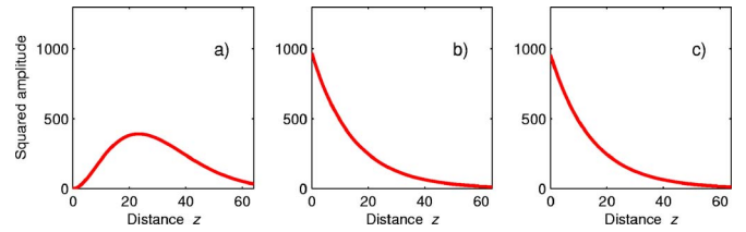
FIG. 11. (Color online) Destructive interference of the two Bloch components of the transmitted wave inside semi-infinite photonic crystal. The frequency is \omega = \omega_d + 10^{-5}c/L , which is just above the degenerate band edge in Fig. 15(b). (a) The squared modulus of the resulting transmitted field—its amplitude at z=0 is small enough to satisfy the boundary conditions (4); (b) and (c) the squared moduli of the two evanescent contributions; both decay with the distance z . The amplitude of the incident wave is unity. Similar graphs related to the frequency just below DBE in Fig. 15(b) are shown in Fig. 10.
