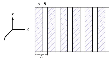
FIG. 7. (Color online) Periodic layered structure with two layers A and B in a primitive cell L . The A layers (hatched) are anisotropic with one of the principle axes of the dielectric permittivity tensor making an oblique angle with the normal z to the layers ( \epsilon_{xz} \neq 0 ). The B layers are isotropic. The x - z plane coincides with the mirror plane of the stack. This structure can support axial dispersion relation \omega(k_z) with stationary inflection point (44), provided that k_x, k_y \neq 0 .
