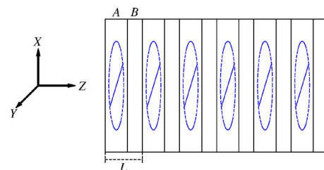
FIG. 8. (Color online) Periodic layered structure with two layers A and B in a unit cell L . The A layer has inplane anisotropy (76), while the B layer can be isotropic. This stack can display axial dispersion relation \omega(k_z) with a degenerate band edge (45), provided that k_x, k_y \neq 0 .
