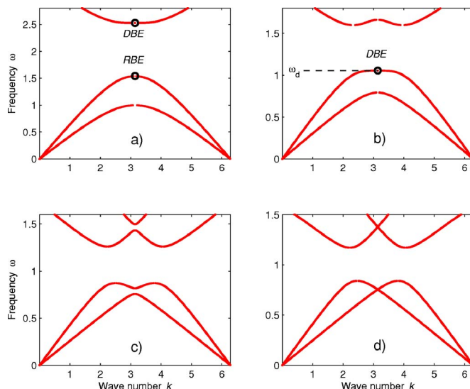
FIG. 15. (Color online) k - \omega diagram of the periodic stack in Fig. 6 for four different values of the B -layer thickness. (a) B/L = 0.71144 , in this case the upper edge of the frequency gap develops a DBE. (b) B/L = 0.37443 , in this case the lower edge of the frequency gap develops a DBE. (c) B/L = 0.1 . (d) B/L = 0 , in this case the intersecting dispersion curves correspond to the Bloch waves with different symmetries—the respective modes are decoupled.
