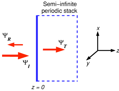
FIG. 1. (Color online) Plane wave normally incident on a semi-infinite photonic crystal. The subscripts I , R , and T refer to the incident, reflected and transmitted waves, respectively. In all cases, the amplitude of the incident wave is unity.
