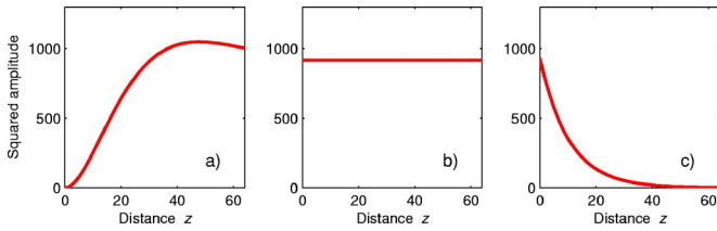
FIG. 10. (Color online) Destructive interference of the two Bloch components of the transmitted wave inside semi-infinite photonic crystal. The frequency is \omega = \omega_d - 10^{-4}c/L , which is slightly below the degenerate band edge in Fig. 15(b). (a) The squared modulus of the resulting transmitted field—its amplitude at z=0 is small enough to satisfy the boundary conditions (4); (b) the squared modulus of the propagating contribution, which is independent of z ; (c) the squared modulus of the evanescent contribution, which decays with the distance z . The amplitude of the incident wave is unity. Similar graphs related to the stationary inflection point are shown in Fig. 9.
