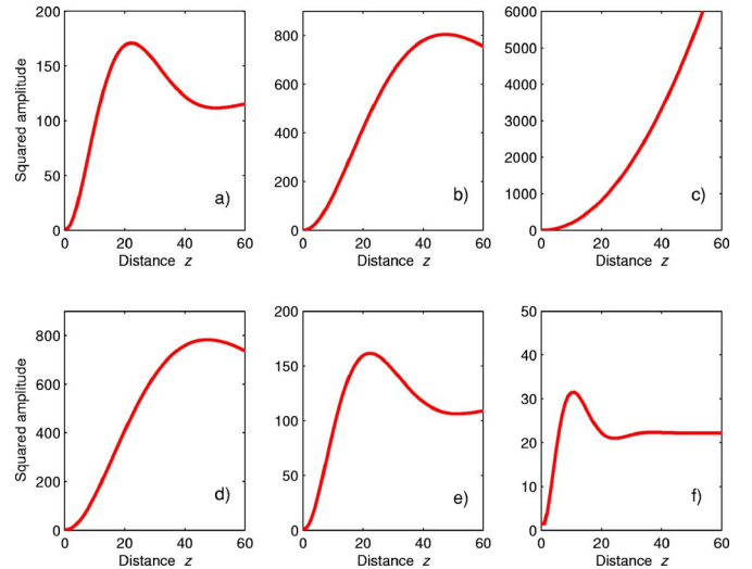
FIG. 3. (Color online) Smoothed profile of the frozen mode at six different frequencies in the vicinity of stationary inflection point: (a) \omega = \omega_0 - 10^{-4}c/L , (b) \omega = \omega_0 - 10^{-5}c/L , (c) \omega = \omega_0 , (d) \omega = \omega_0 + 10^{-5}c/L , (e) \omega = \omega_0 + 10^{-4}c/L , (f) \omega = \omega_0 + 10^{-3}c/L . In all cases, the incident wave has the same polarization and unity amplitude. The distance z from the surface of semi-infinite photonic crystal is expressed in units of L . Physical parameters of the periodic structure are specified in (78) and (79).
