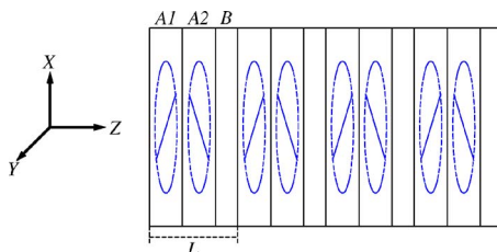
FIG. 6. (Color online) Periodic stack capable of supporting k-\omega diagram with a DBE. A unit cell L includes three layers: two birefringent layers A_1 and A_2 with misaligned in-plane anisotropy, and one isotropic B layer. In order to support a DBE, the misalignment angle \phi between adjacent anisotropic layers A_1 and A_2 must be different from 0 and \pi/2 . A detailed description of this periodic structure is given in Sec. V.
