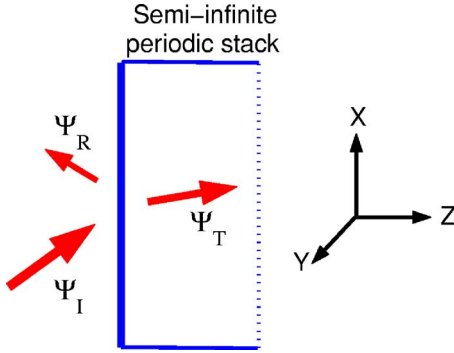
FIG. 12. (Color online) Scattering problem for a plane wave obliquely incident on a semi-infinite periodic layered medium. The arrows schematically shows the Pointing vectors of the incident, reflected and transmitted waves. The amplitude of the incident wave is unity.
