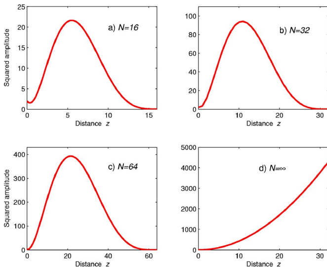
FIG. 5. (Color online) Smoothed profile of the frozen mode in periodic layered structures composed of different number N of unit cells L . The frequency is equal to that of the degenerate band edge. The initial rate of growth of the frozen mode amplitude is virtually independent of N and described by (34). The limiting case (d) of the semi-infinite structure is also shown in Fig. 4(c). In all cases, the incident wave has the same polarization and unity amplitude. The distance z from the surface is expressed in units of L .
