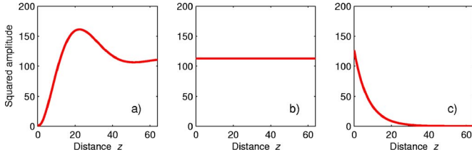
FIG. 9. (Color online) Destructive interference of the propagating and evanescent components of the transmitted wave inside semi-infinite photonic crystal. The frequency is close but not equal to that of stationary inflection point. (a) The squared modulus of the resulting transmitted field—its amplitude at z=0 is small enough to satisfy the boundary conditions (4); (b) the squared modulus of the propagating contribution, which is independent of z ; (c) the squared modulus of the evanescent contribution, which decays with the distance z . The amplitude of the incident wave is unity. The distance z from the surface is expressed in units of L .
