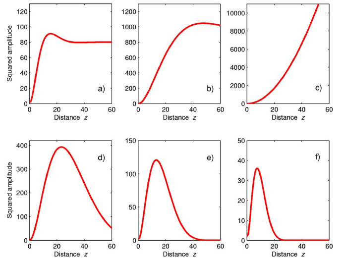
FIG. 4. (Color online) Smoothed profile of the frozen mode at six different frequencies in the vicinity of degenerate band edge: (a) \omega = \omega_d - 10^{-4}c/L , (b) \omega = \omega_d - 10^{-6}c/L , (c) \omega = \omega_d , (d) \omega = \omega_d + 10^{-6}c/L , (e) \omega = \omega_d + 10^{-5}c/L , (f) \omega = \omega_d + 10^{-4}c/L . In the transmission band (at \omega < \omega_d ), the asymptotic field value diverges as \omega \rightarrow \omega_d . By contrast, in the band gap (at \omega > \omega_d ), the asymptotic field value is zero. The amplitude of the incident wave at z < 0 is unity. The distance z from the surface is expressed in units of L . Physical parameters of the periodic structure used in computations are specified in Sec. V.
